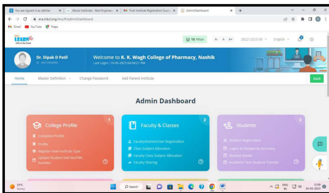
Admin Dashboard
