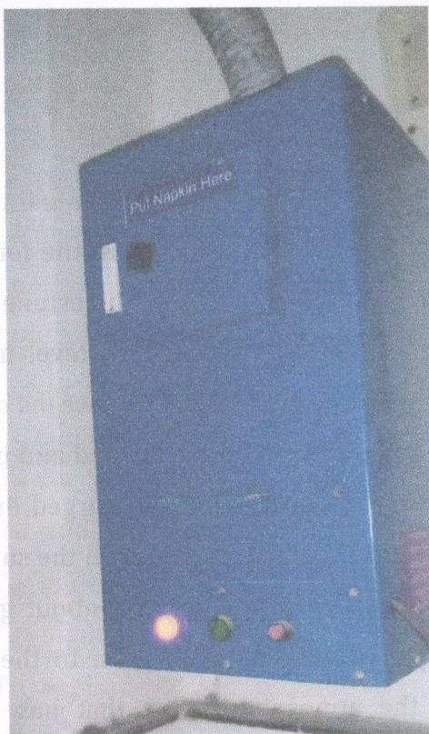
Fig 4.: Sanitary Napkin Disposal Machine
