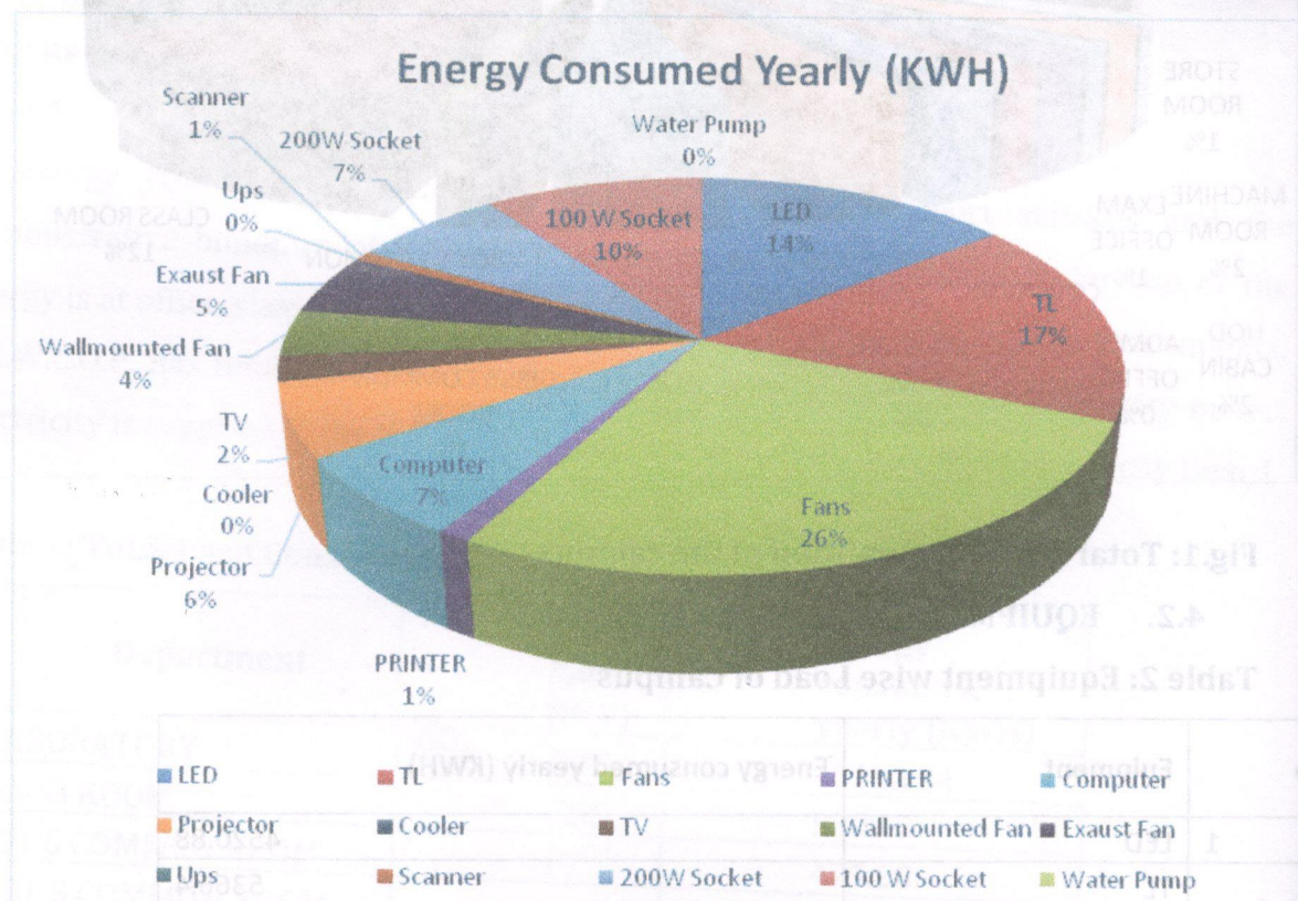
Fig.2.: Equipment wise energy consumed yearly chart
