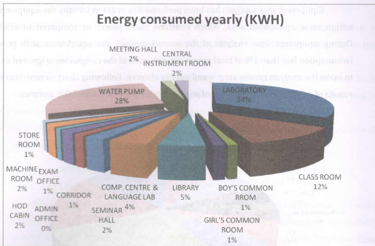
Fig.1: Total Load consumption of the campus
