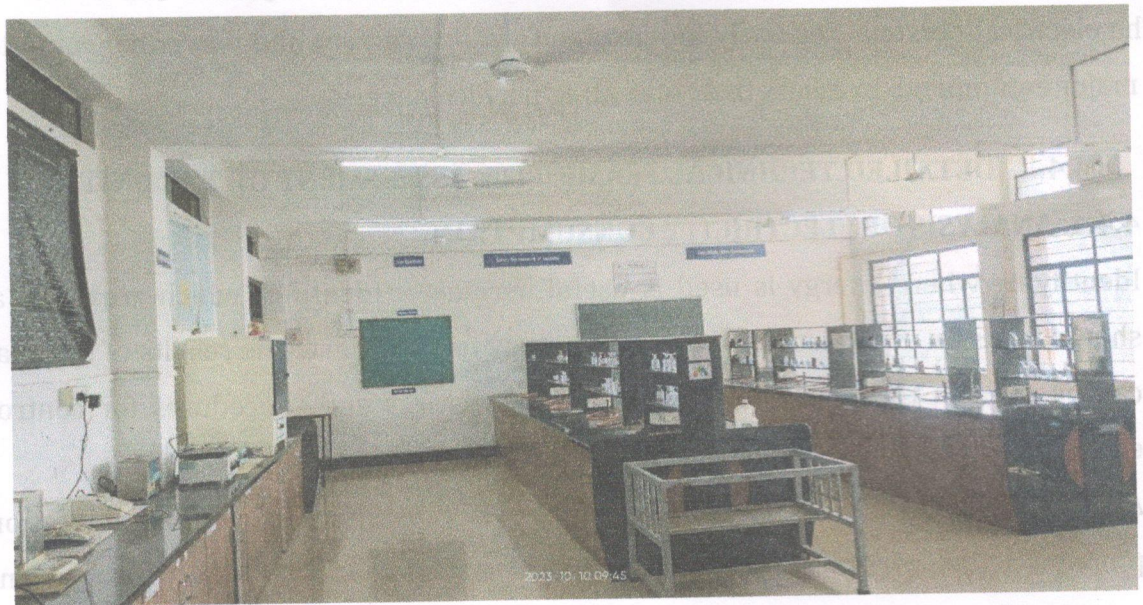
Fig. 3. : Conventional Ballast FTL
